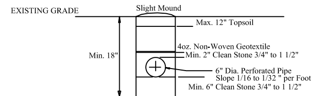
Absorption Trench Detail NTS
