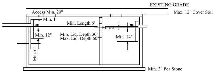
L/W Ration >2 but <4 Septic Tank Detail NTS
