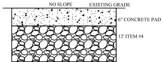
Equipment Parking Detail NTS
