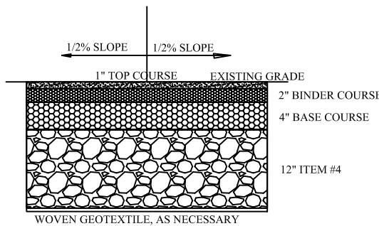
Entrance/Exit Pavement Detail NTS
