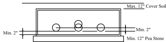
Note: Outlet at Same Elevation Distribution Box Detail NTS
