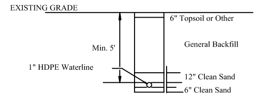
Waterline Detail NTS
