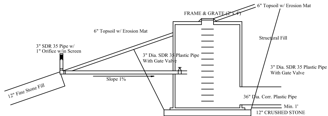
8' Diameter Manhole Detail NTS
