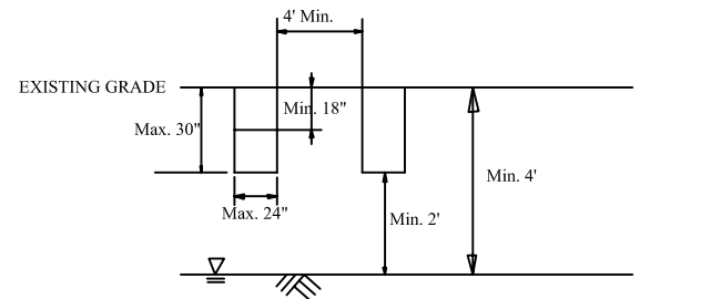
Absorption Field Detail NTS
