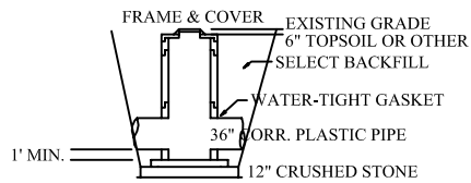
4' Diameter Manhole Detail NTS
