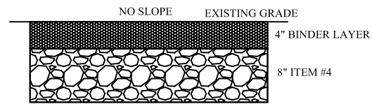
Plant Area Pavement NTS
