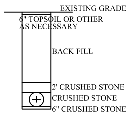
NOTE: CHECK MANUFACTURER SPECIFICATIONS Culvert Bedding Detail NTS
