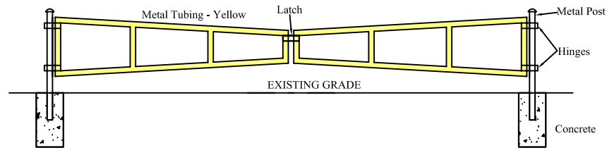
Gate Detail NTS
